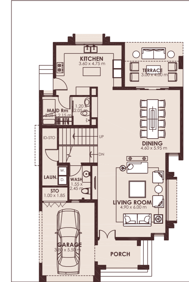
A - GROUND FLOOR PLAN
