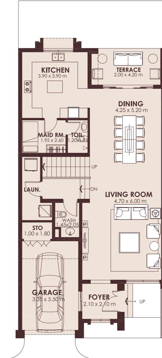
A - GROUND FLOOR PLAN
