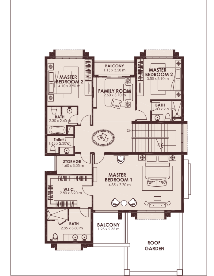
B - FIRST FLOOR PLAN
