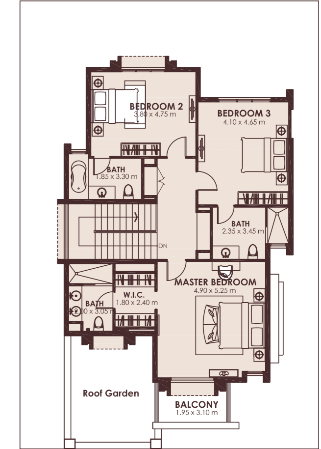
B - FIRST FLOOR PLAN
